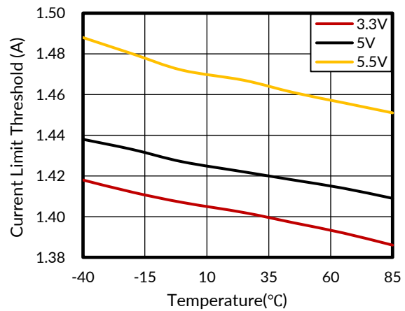
Figure 9. Current Limit Threshold vs Temperature
