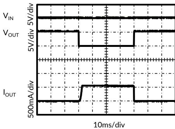
Figure 17. No Load into Short-Circuit
