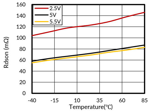
Figure 7. High-side MOSFET On Resistance vs Temperature
