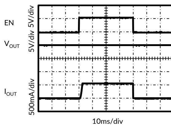
Figure 18. Device Enabled into Short-Circuit
