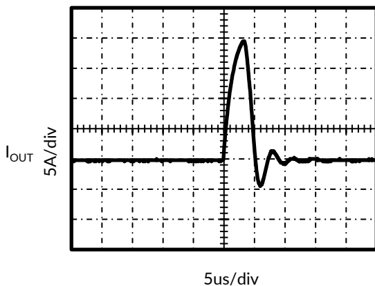
Figure 19. Short-Circuit Response Time
